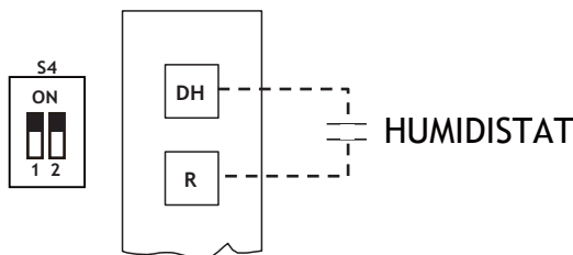
S4-2 DIP switch
